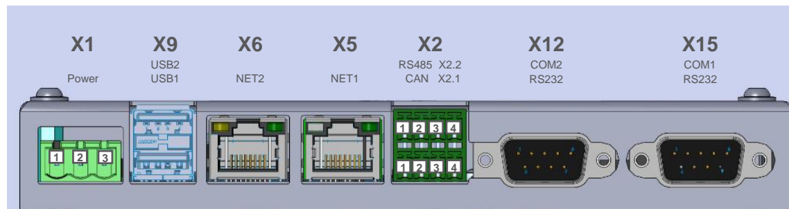
Figure 2: Interfaces bottom view of Control Panels CP-101g 3x-xx30
