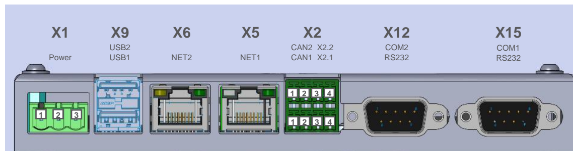
Figure 3: Interfaces bottom view of Control Panels CP-101g 3x-xx40
