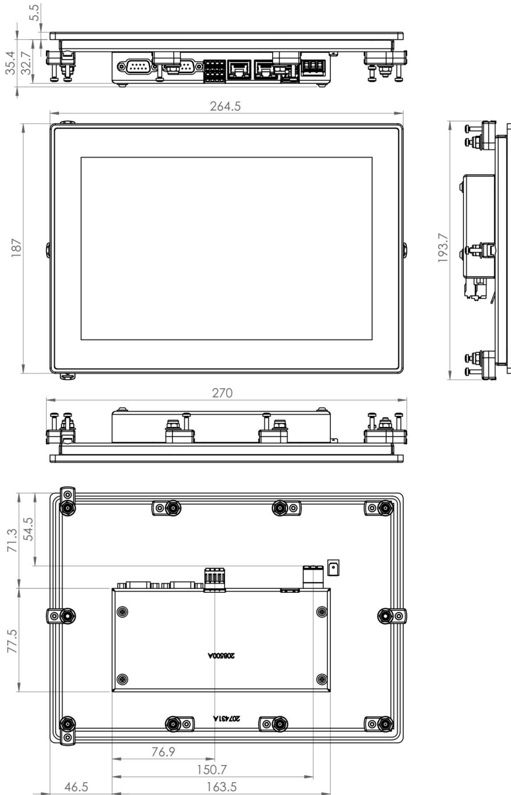
Figure 7: Dimension drawings
