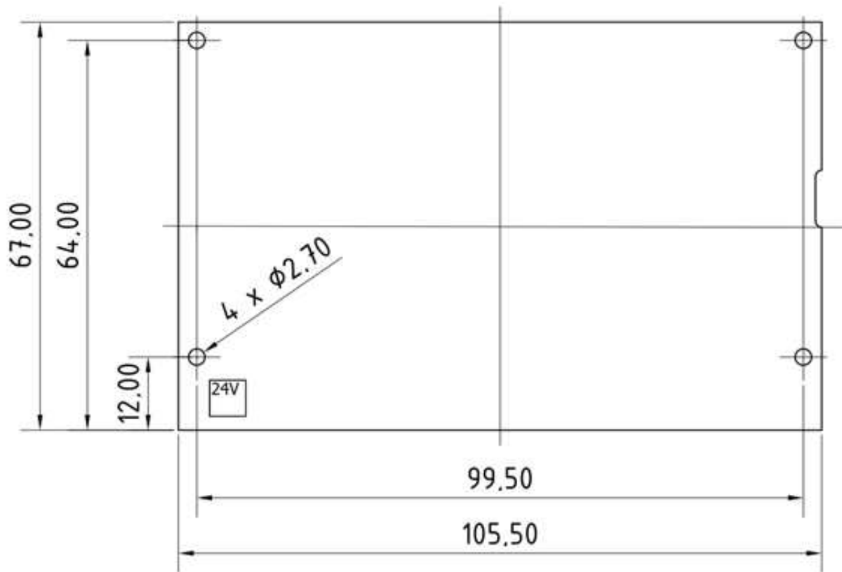
Figure 2: Dimensions (Measurements in Millimetres)
