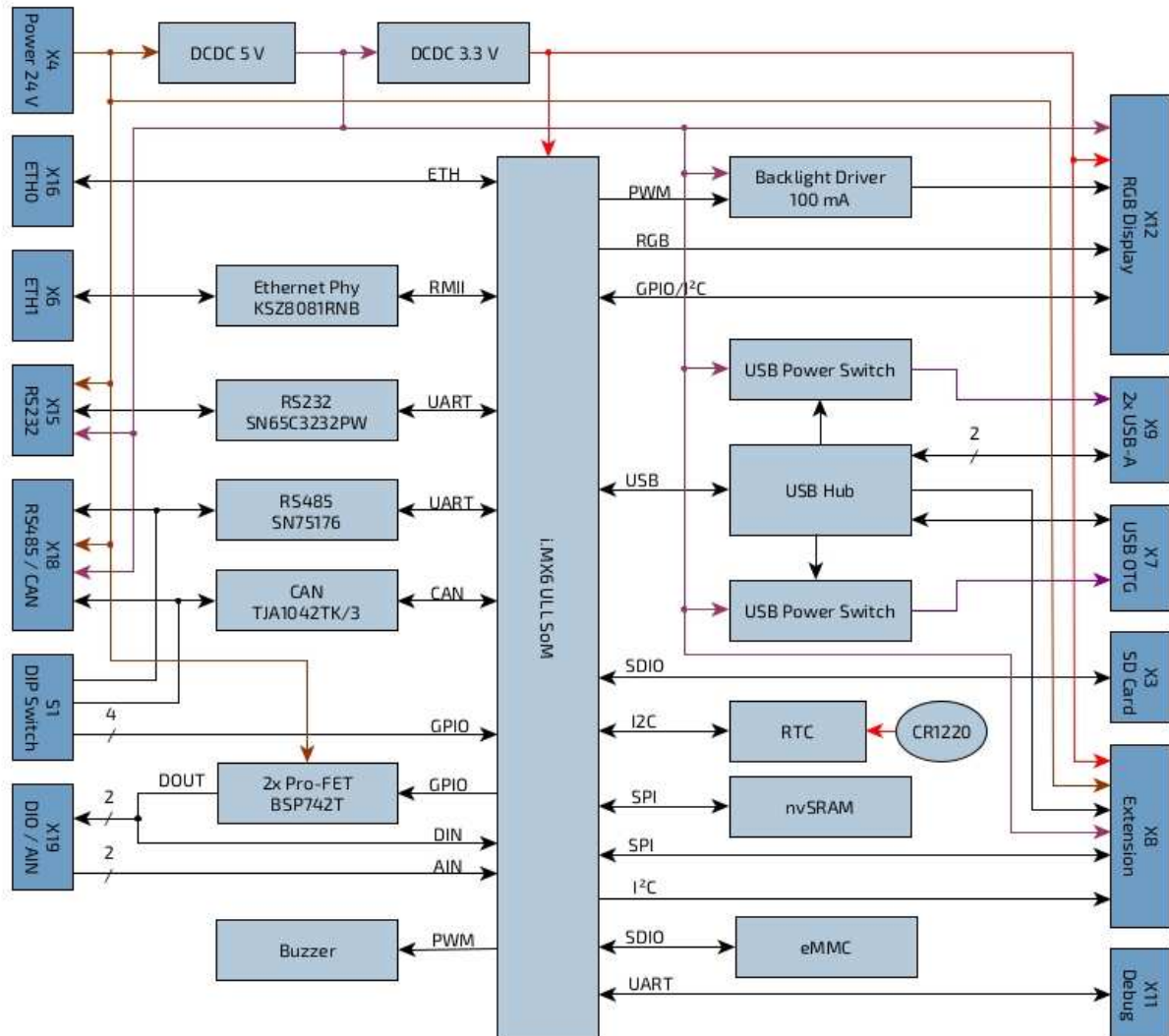
Figure 3: Block Diagram
