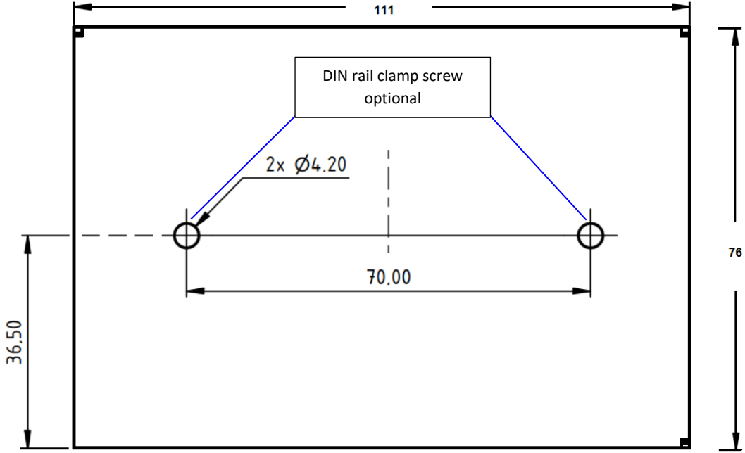
Figure 2: Bottom view
