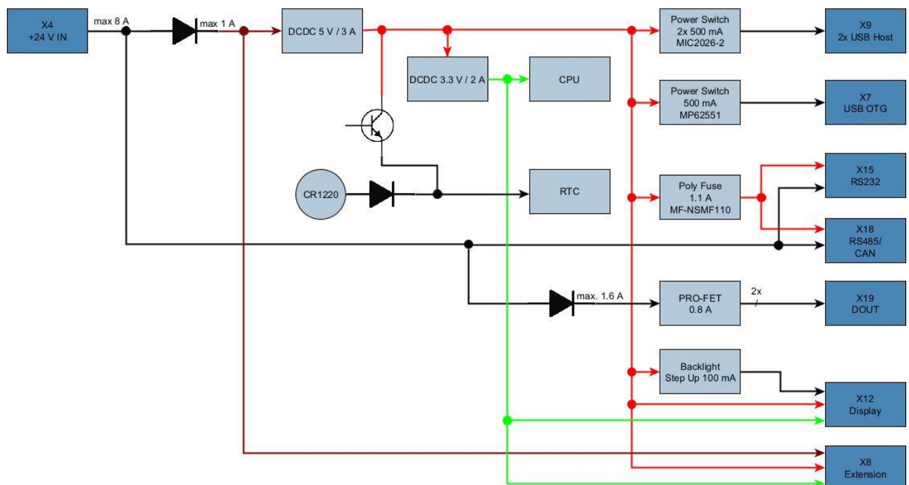
Figure 6: Power Tree
