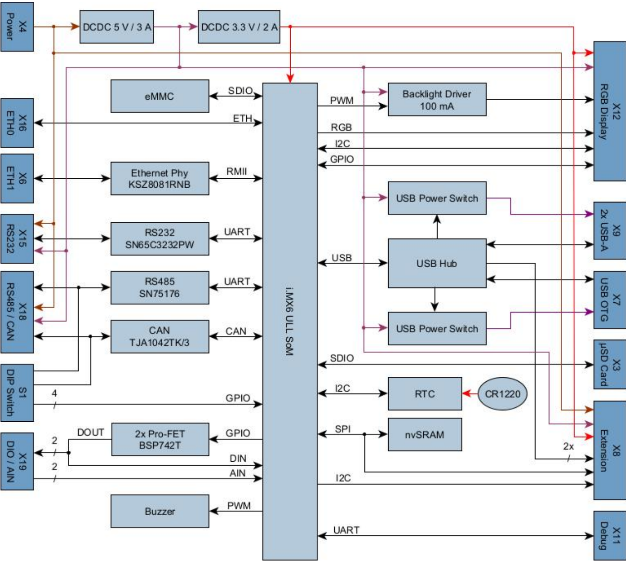
Figure 7: Block Diagram
