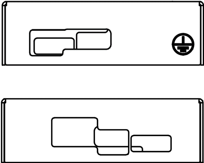
Figure 5: Side views
